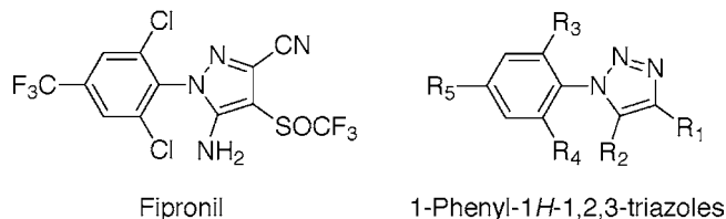
Figure 1. Structures of fipronil and 1-phenyl-1 H -1,2,3-triazoles.
