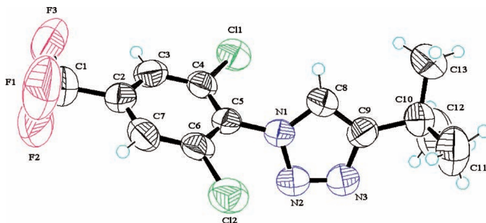
Figure 2. X-ray crystal structure of 9 .
