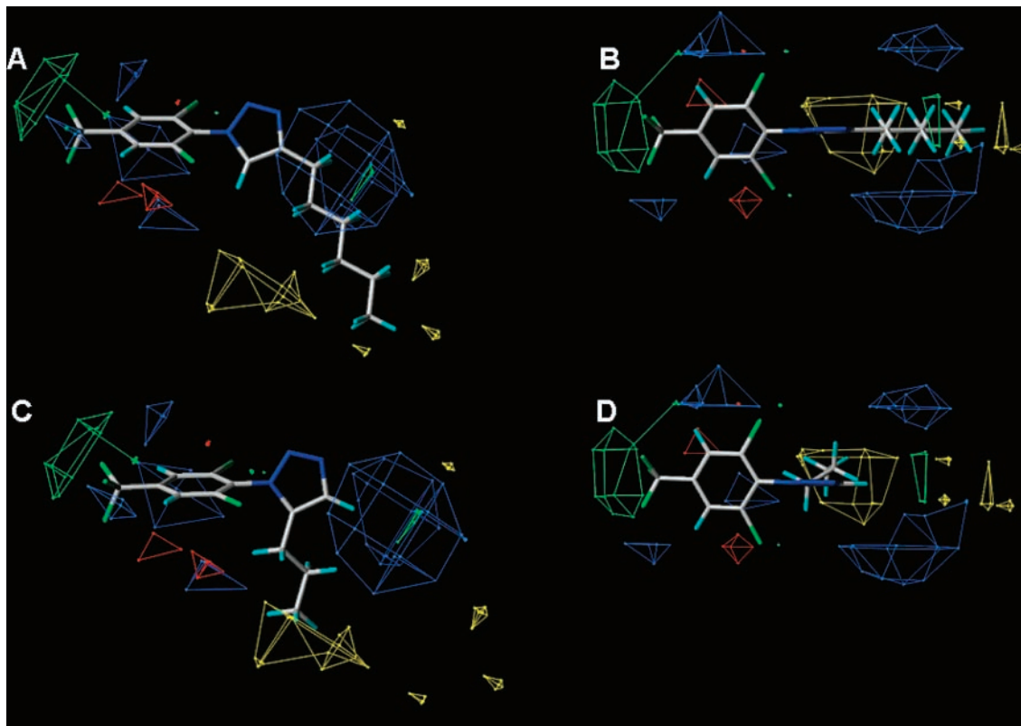
Figure 6. CoMFA contour maps showing the results of analyses of the human \beta 3 GABA receptor: (A, B) orthogonal views of maps with 3 ; (C, D) orthogonal views of maps with 12 .
