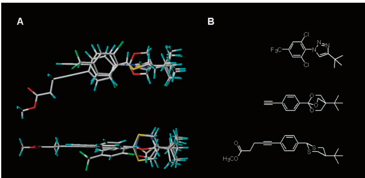
Figure 9. Superimposition of three representative heterocyclic GABA antagonists: (A) orthogonal views of the superimposed molecules; (B) structures of the superimposed molecules.
