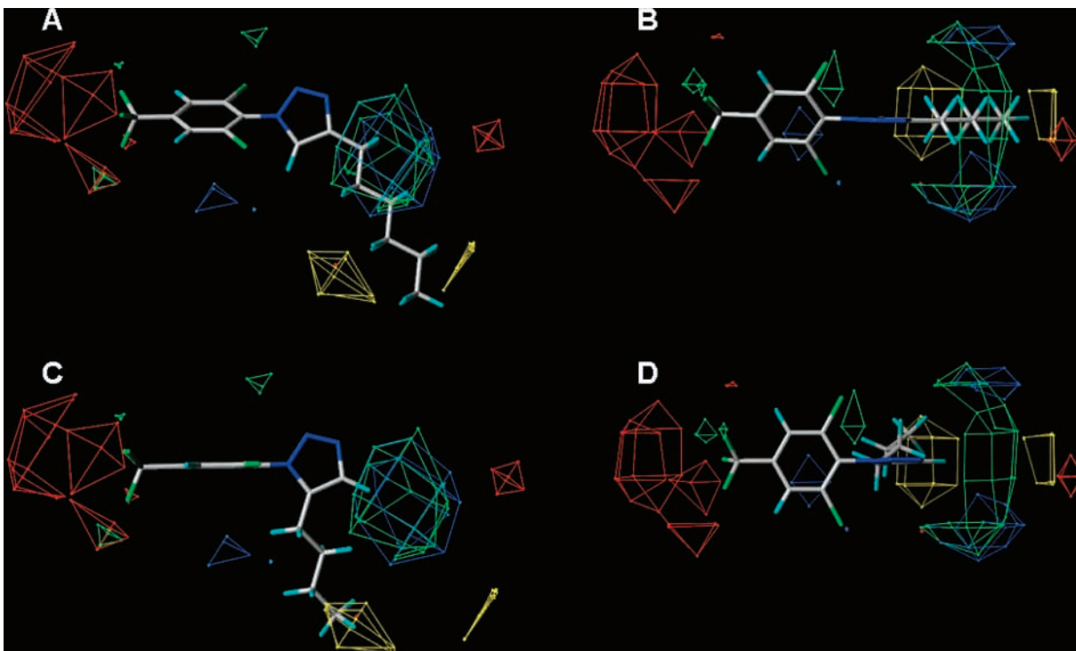
Figure 7. CoMFA contour maps showing the results of analyses of the housefly GABA receptor: (A, B) orthogonal views of maps with 3; (C, D) orthogonal views of maps with 8.
