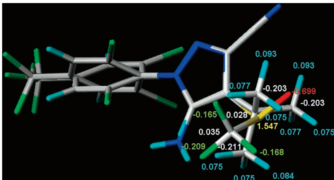
Figure 10. Superimposition of fipronil on 9 . Numbers indicate the electric charges on the atoms.
